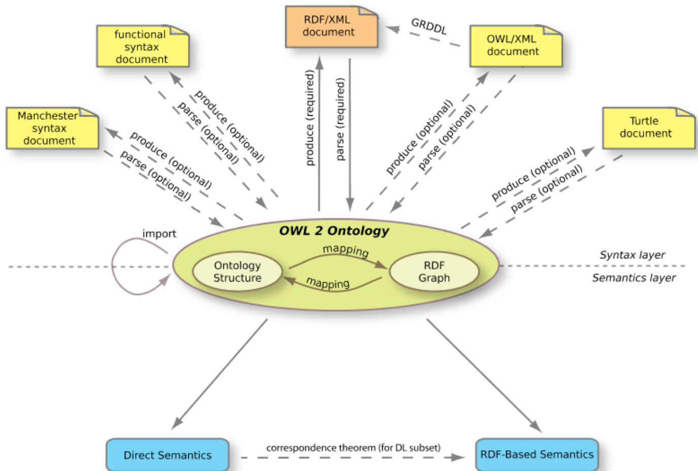
Figure 1. The Structure of OWL 2
